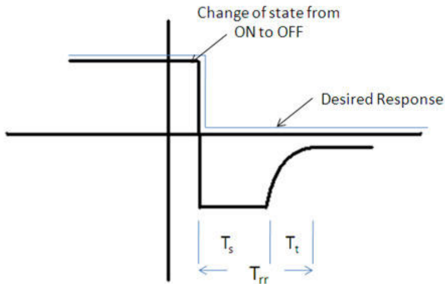
Characteristics of Diode switching time
